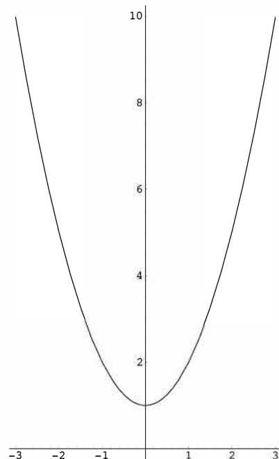
Equation X = x^2 + 1 :
