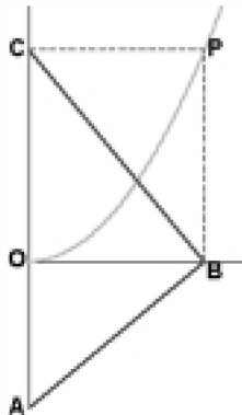
Combining a number of these triangles creates the parabola
