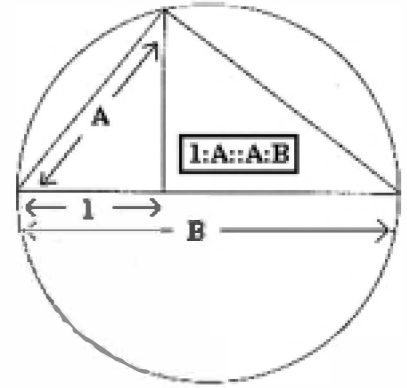
One mean between two extremes, inside the circle.
