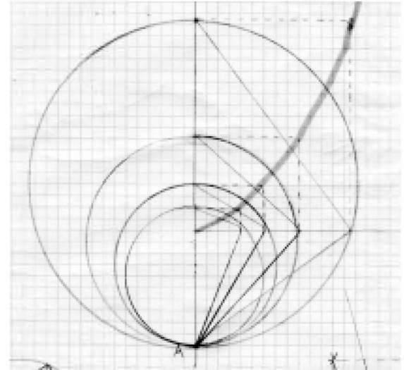
Combining a number of these triangles creates the parabola
