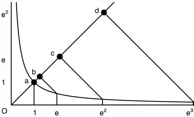
FIGURE 5a Projection of Equal Hyperbolic Areas
