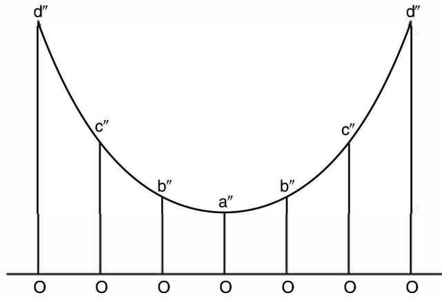
FIGURE 5d The Relationship Between Hyperbola and Catenary
