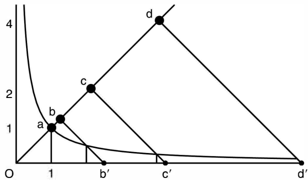
FIGURE 5b Measuring the Lengths Along the Axis
