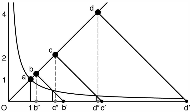
FIGURE 5c The Relationship Between Hyperbola and Catenary
